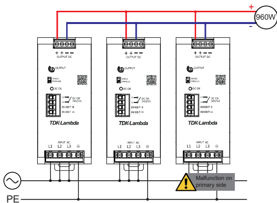
Fig. 35: Connection scheme of n+1 power supplies paralleled for the purpose of a 960W limited redundancy
