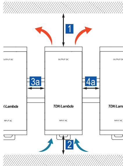
Fig. 26: Installation clearances to heat sources
