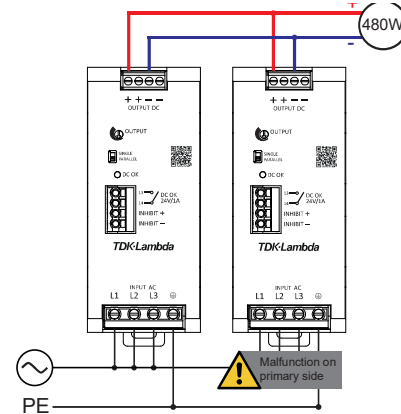
Fig. 36: Connection scheme of 1+1 power supplies paralleled for the purpose of a 480W limited redundancy
