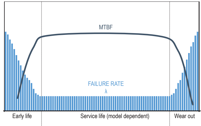
Fig. 23: Generic diagram visualising failure rate and MTBF values during the products life-cycle
