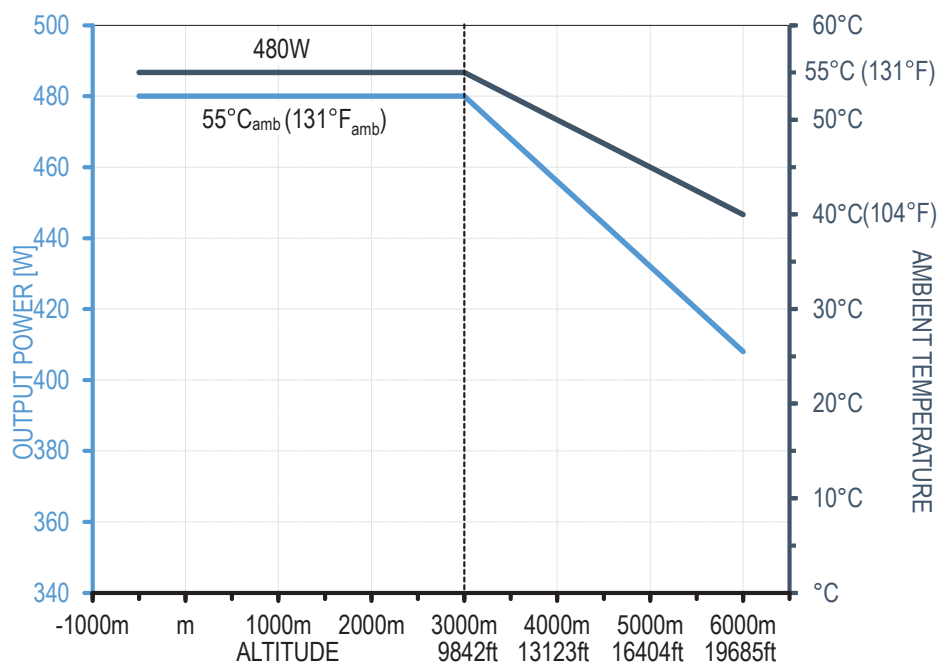
Fig. 11: Output power or ambient temperature derating at increasing altitudes
