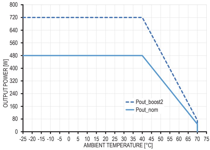
Fig. 14: Power deratings in mounting positions Fig. 17 - Fig. 21
