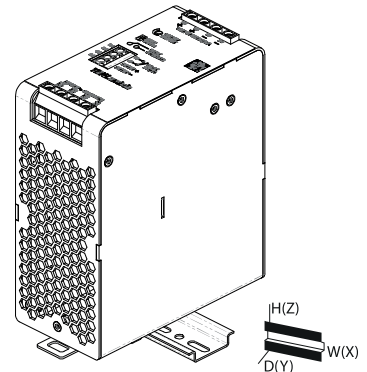
Fig. 21: Back side down
