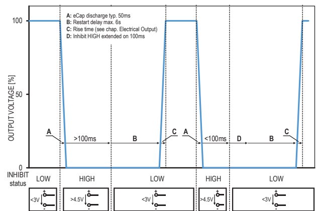
Fig. 29: Control of the output voltage in dependence of the inhibit relay status.
