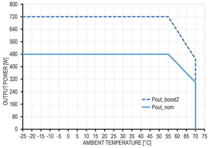
Fig. 12: Power deratings in mounting positions Fig. 16
