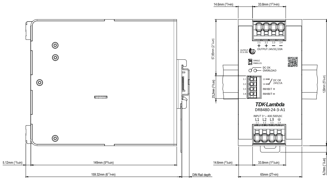
Fig. 25: Dimension drawing of DRB480-24-3-A1
