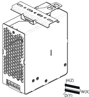
Fig. 20: Front side down
