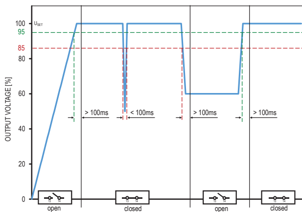
Fig. 28: DC-OK relay characteristic in dependence of output voltage changes
