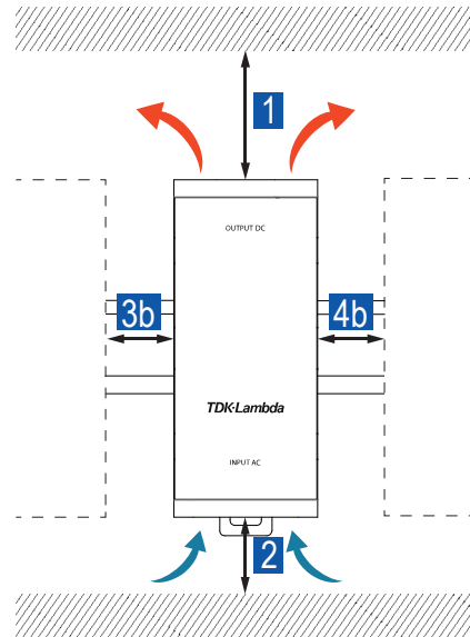
Fig. 27: Installation clearances to passive components
