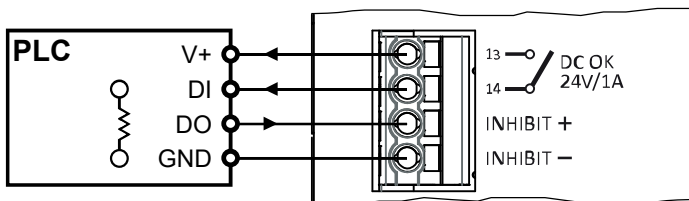
Fig. 30: Generic connection diagram of DC OK and INHIBIT contacts
