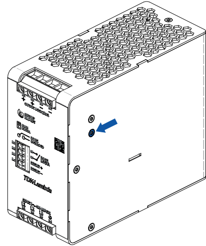
Fig. 32: Position of the connection screw for the GDT
