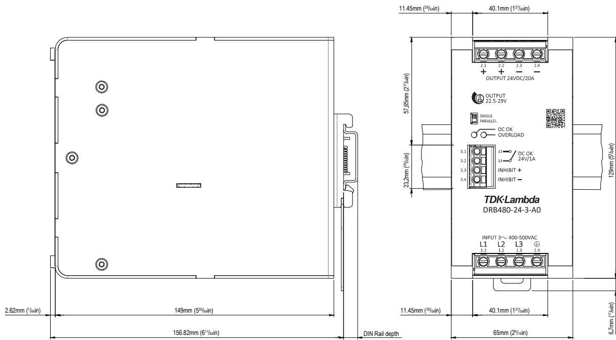
Fig. 24: Dimension drawing of DRB480-24-3-A0
