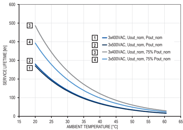
Fig. 22: Power supply service lifetime in dependence of ambient temperature
