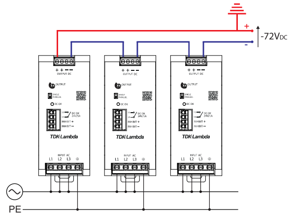
Fig. 39: Connection scheme for series operation with negative voltage level
