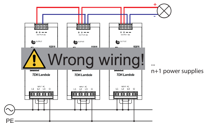
Fig. 34: Example of a wrong connection scheme
